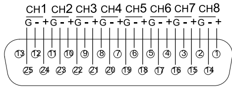
DB-25 TASCAM PINOUT
